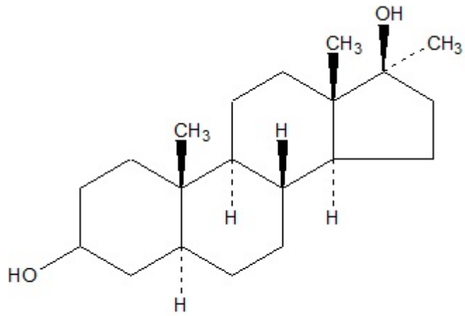
17 \alpha -Methyl-5 \alpha -androstane-3,17 \beta -diol
